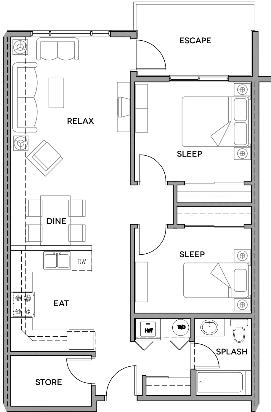
3 UNIT E1 PLAN [780 ft 2 NET] A3.3 1/4"=1'-0"
