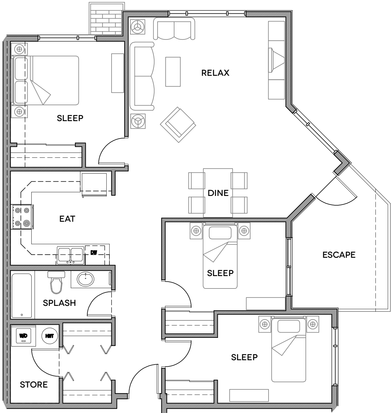
3 UNIT D PLAN [1160 ft 2 NET] A3.2 1/4"=1'-0"
