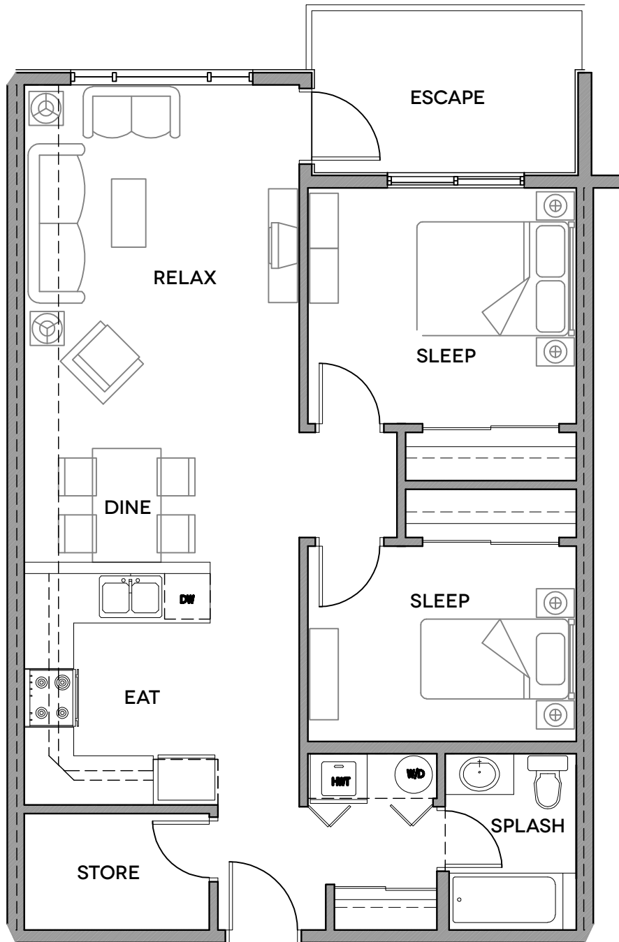
2 UNIT E PLAN [846 ft 2 NET] A3.3 1/4"=1'-0"
